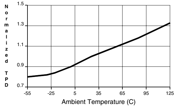
NORMALIZED TCO vs. TEMPERATURE
